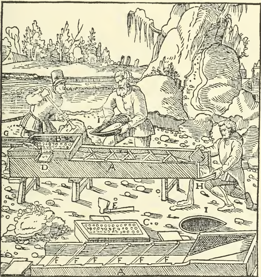
A—SLUICE. B—BOX. C—BOTTOM OF INVERTED BOX. D—OPEN PART OF IT. E—IRON HOE. F—RIFFLES. G—SMALL LAUNDER. H—BOWL WITH WHICH SETTLINGS ARE TAKEN AWAY. I—BLACK BOWL IN WHICH THEY ARE WASHED.
